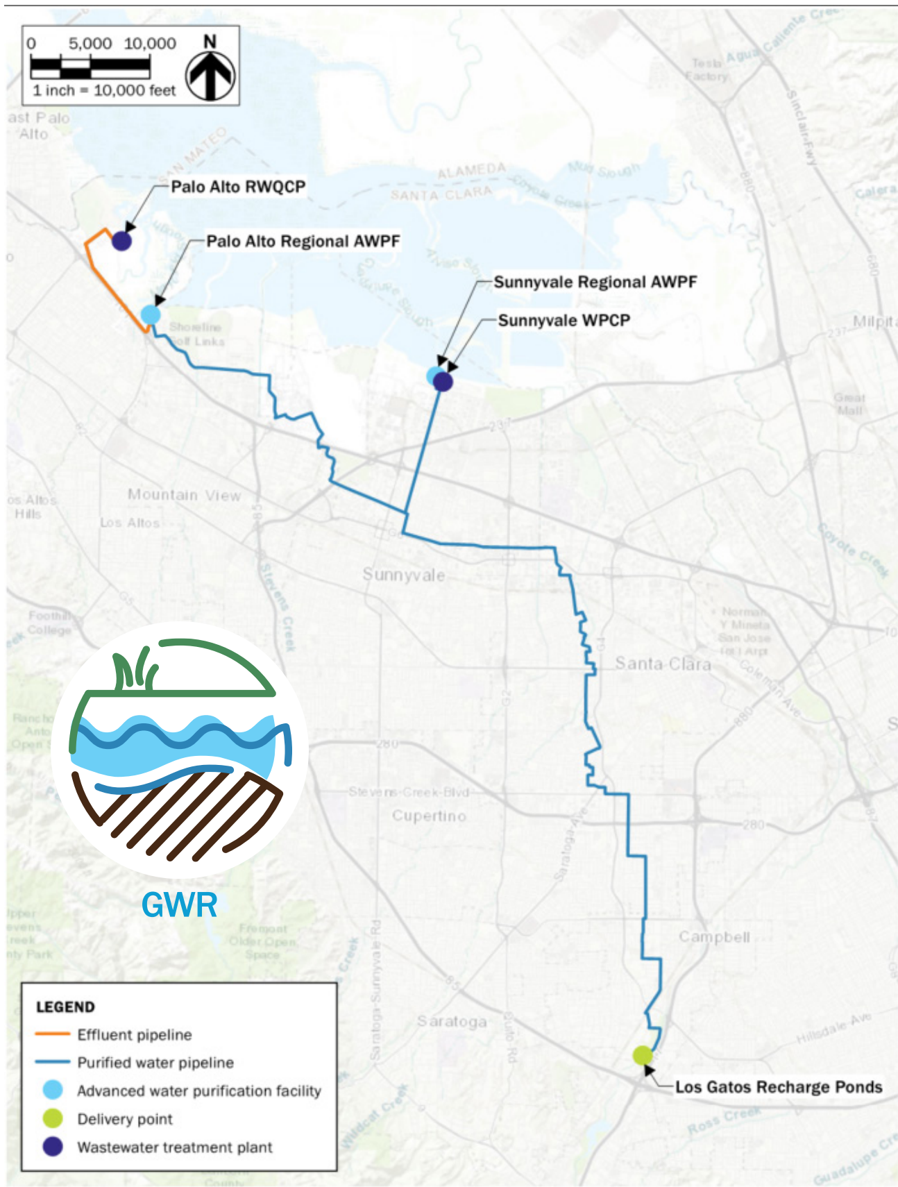
Figure 6-7. Portfolio 4: PA/SV GWR facility locations and pipeline alignments
